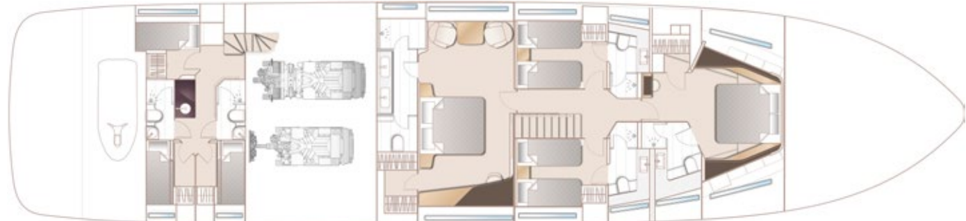
LOWER DECK WITH OPTIONAL MASTER STATEROOM BREAKFAST AREA AND 3 CABIN/2 HEAD CREW ACCOMMODATION
